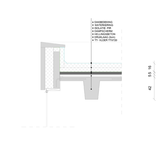
DETAIL F
