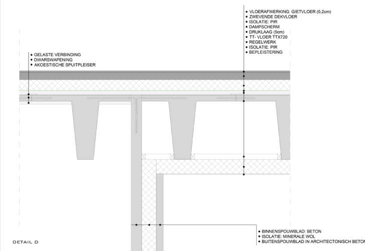
DETAIL D
