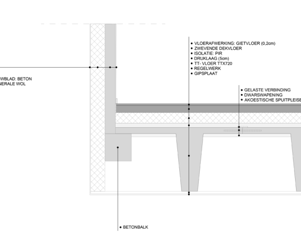
DETAIL E
